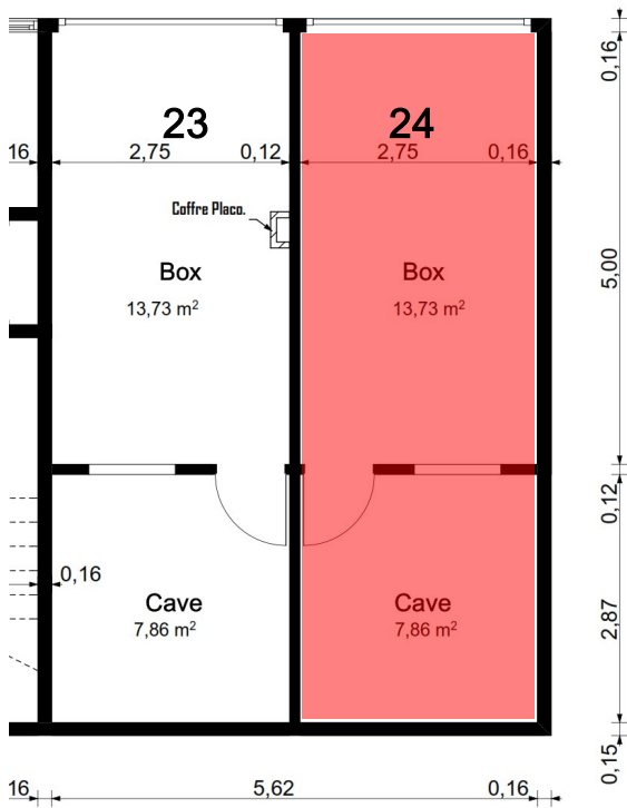
PARKING NIV.-1
