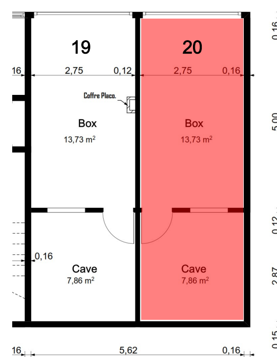
PARKING NIV.-1
